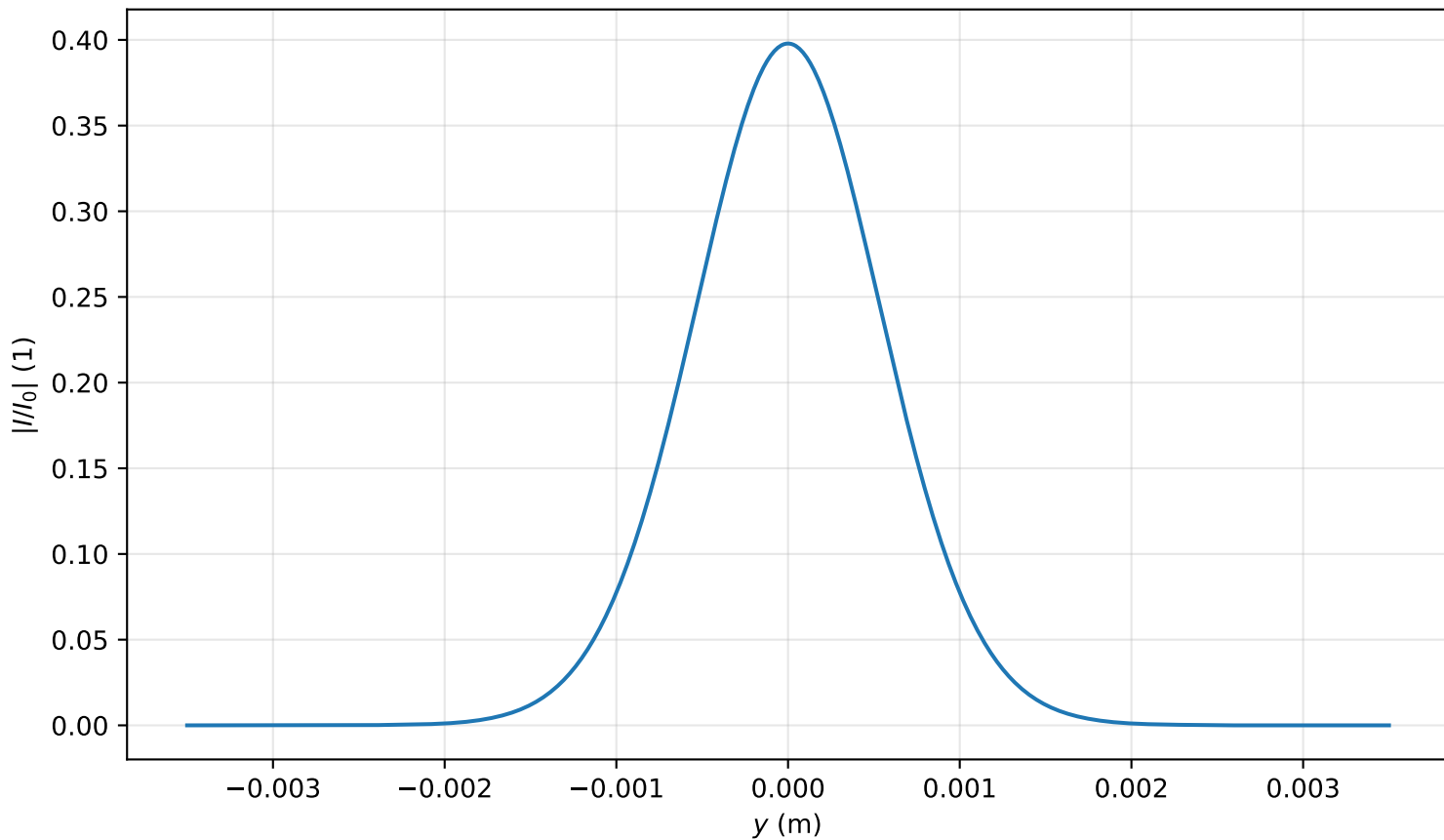
Intensity profile I(x = 0, y, z = 2.866)/I_0 , P_{in}=0.2P_{cr} , artificial time
